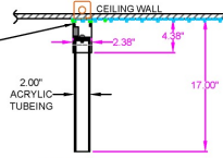
SECTION VIEW "A"-A
