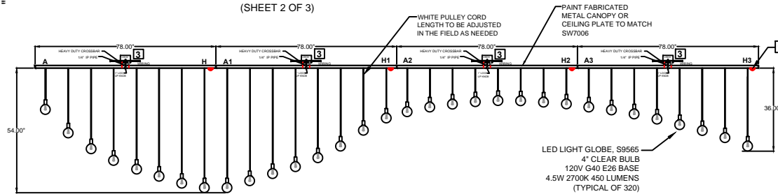
FRONT VIEW (SEE SHEET 3 OF 3)
