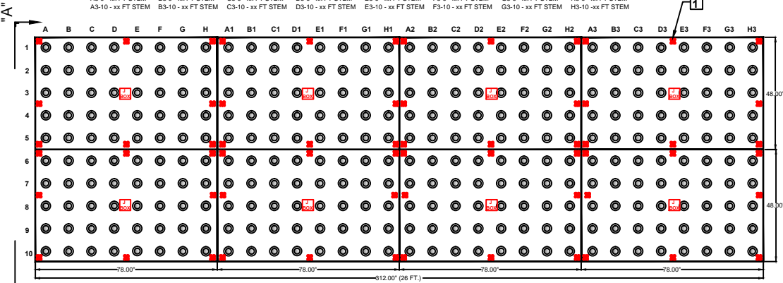
BOTTOM VIEW DETAIL (SHEET 2 OF 3)
