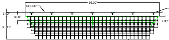
EXAMPLE OF FIXTURE INNER MECHANISM CONNECTION
