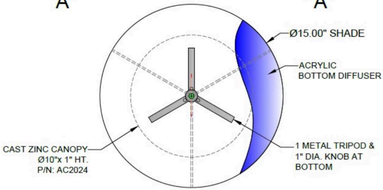
VIEW "A"-"A"
