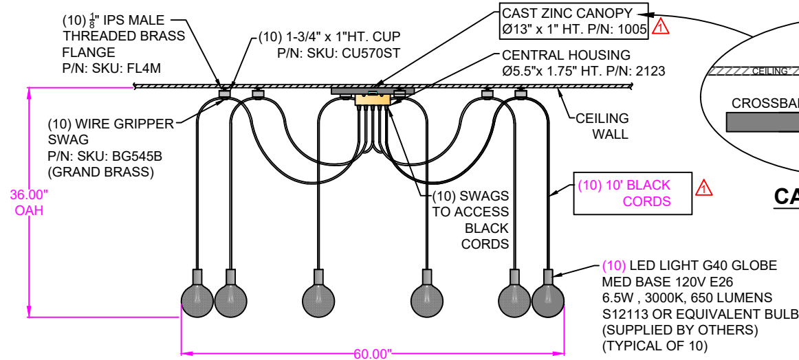
FRONT VIEW
