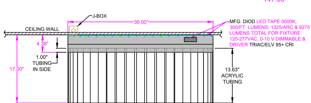
FRONT VIEW
