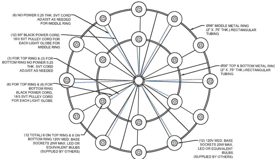
VIEW "A"-A
