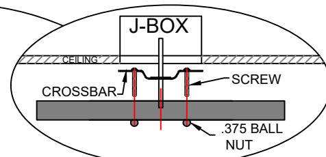
CANOPY ASSY.
