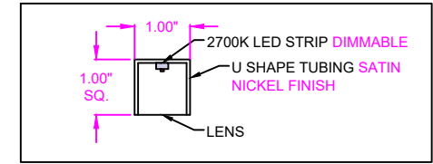
DETAIL "D" SCALE 1:8
