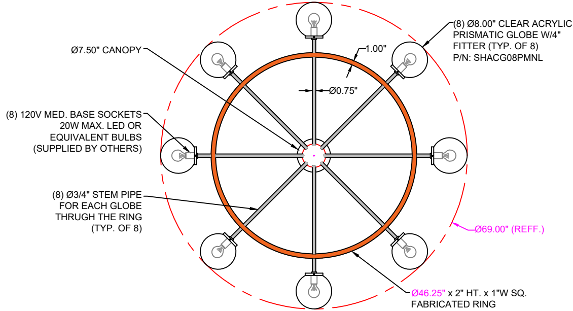
VIEW "A"-A"
